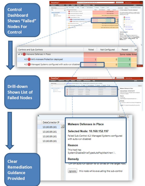
SecureVue- Provides Automated Security Control Monitoring and Remediation Guidance
